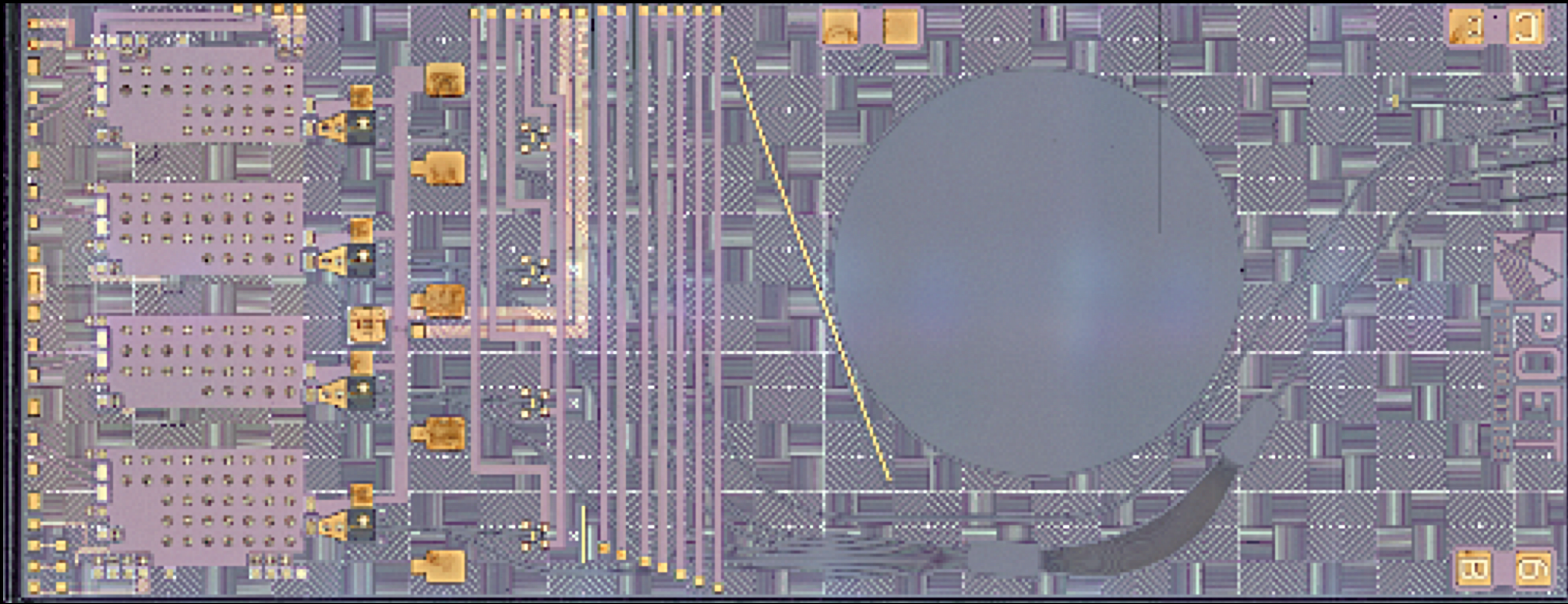
POET Technologies 400G Transmit Optical Engine with integrated drivers, lasers and MPDs
